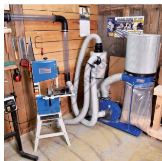
Shown Set Up With Optional Dust Collector
