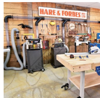
Shown Set Up with Optional Dust Hose and Access
