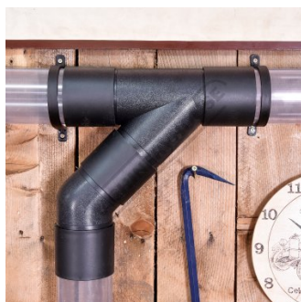
Y Connector Joined to 45 Degree Elbow
