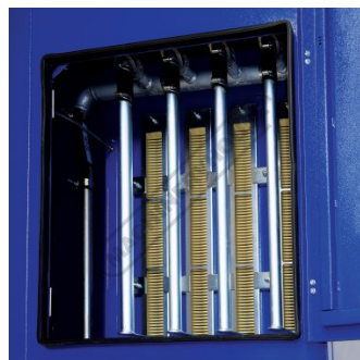
Air Filtration with Jet Pulse Cleaning
