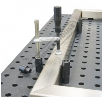
Optional SC 60 Clamp Shown Screwed into Threaded Adaptor View 2
