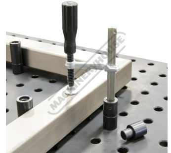
Optional SC 60 Clamp Shown Screwed into Threaded Adaptor
