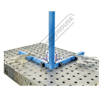
Square Tube Setup with Stops Locking Clamps and Magnetic Squares
