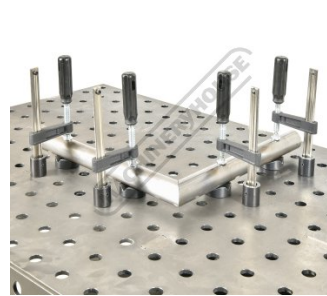
Round Tube Setup with 4 x Clamps and V Pads
