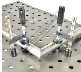
Round Tube Setup with Clamps and V Pads
