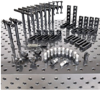
Kit Components
