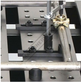
The V Blocks can be placed directly into the holes on the BullPro Table Straight Edge Stop and V Spacer
