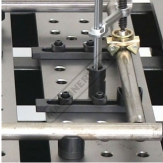
The V Blocks can be placed directly into the holes on the BuildPro Table Straight Edge-Stop and V Spacer
