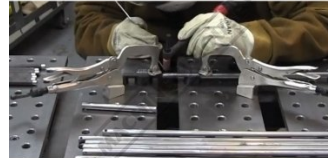
Shown Clamping
