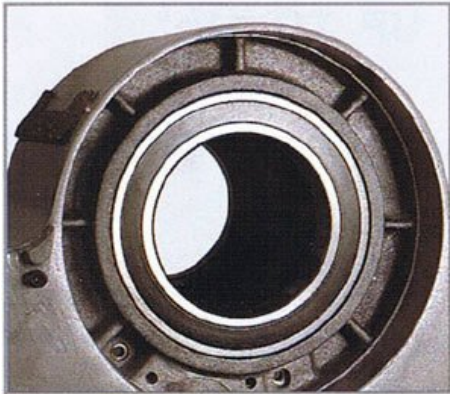
Spindle Support has sealed ball bearings, ensuring continued accuracy through lack of wear.
