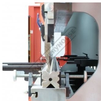
Top and Bottom Tooling
