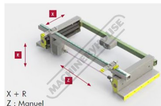
XR Backgauge
