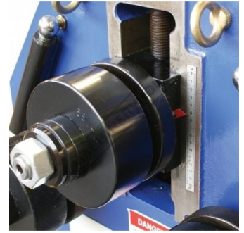
Height Gauge
