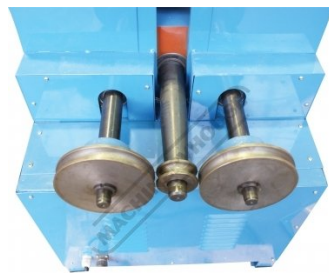
Small Tube Bending Rolls Rear
