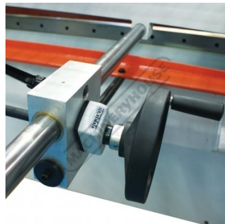
Backgauge Handwheel with Digit Counter
