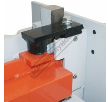
Material Clamp
