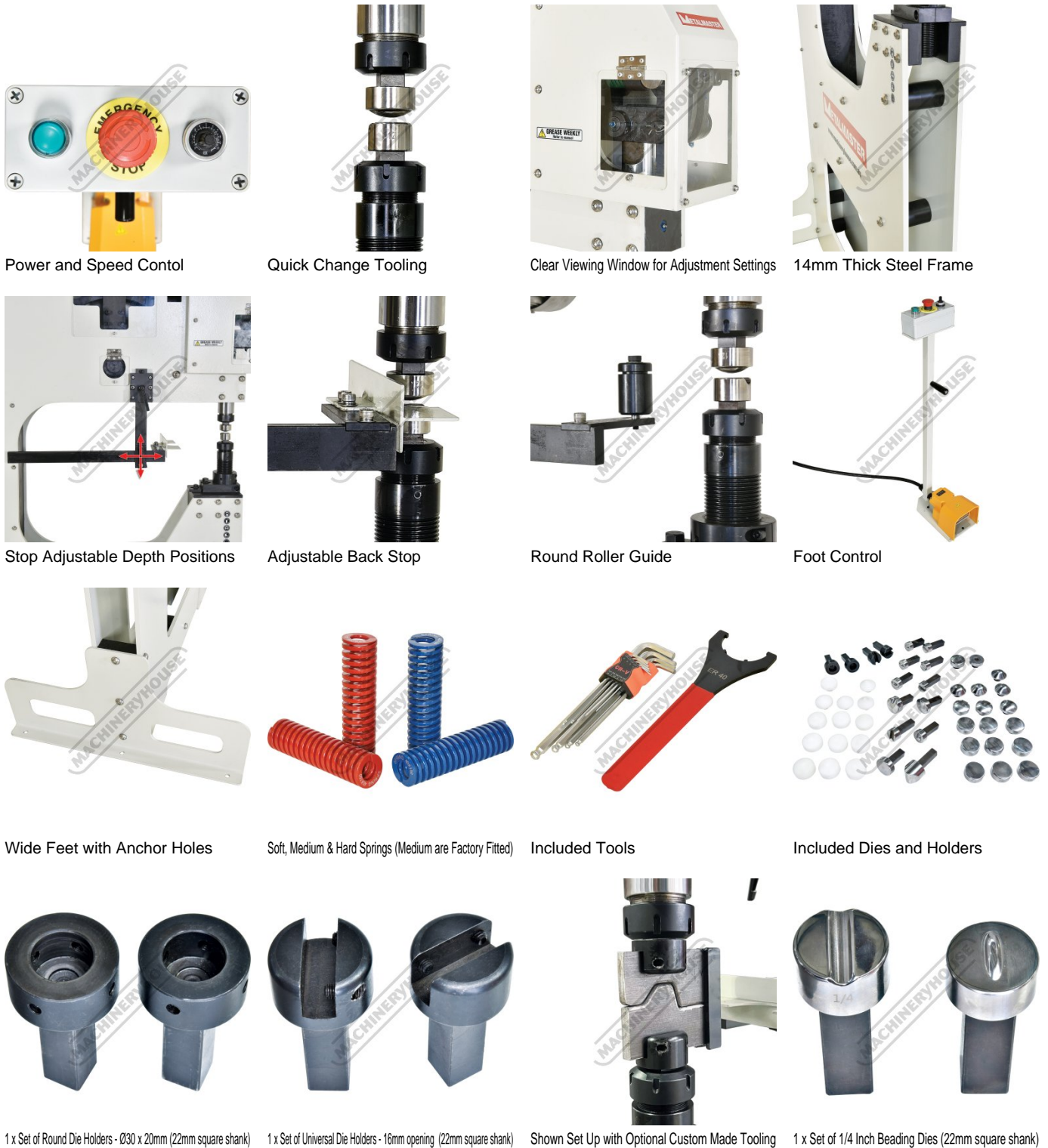
1 x Set of Round Die Holders - Ø30 x 20mm (22mm square shank)
