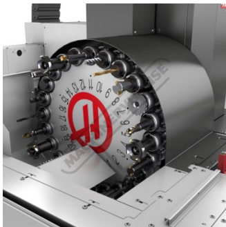
Tool Holder
