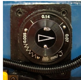
Quill Power Feed Dial
