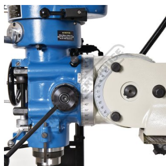
Universal Tilting Rotating Head
