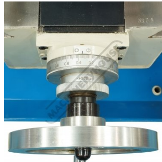
Y-Axis Dial
