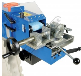
Compound Swivel Vice with Heavy Duty Leadscrew Vice Clamp
