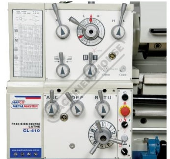
Headstock Controls
