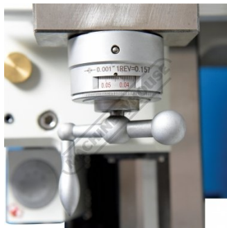
Compound Slide Dial in Imperial Mode
