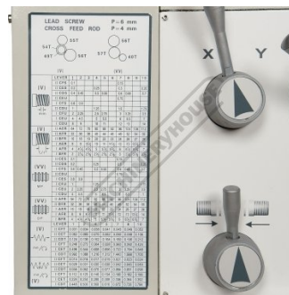
Thread and Feed Chart
