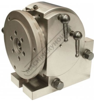
Right View
