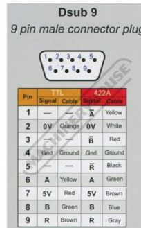
Dsub9 Wiring Diagram
