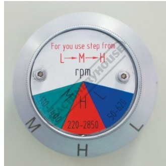
3 Speed Gearbox
