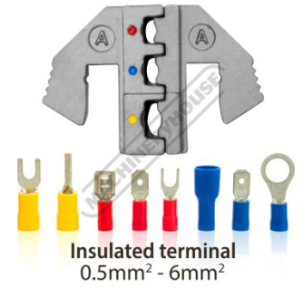
Insulated Terminal Jaw
