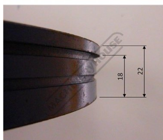
BC175 WHEEL OD 194 BORE 40
