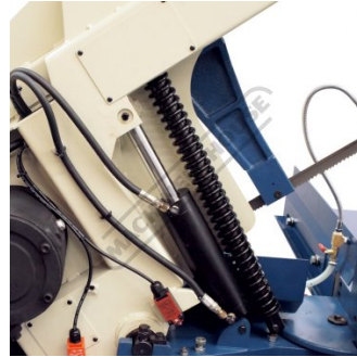
Hydraulic Rise-Fall with Spring Damper
