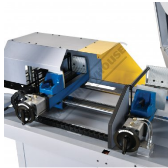
Hydraulic Vice
