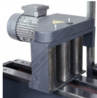
Auto Powered Roller Feed Vice
