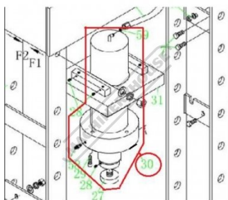
4PR0030 CYLINDER ASSY 30
