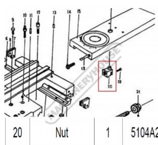
2LX5104 NUT (CROSS) 5104A2
