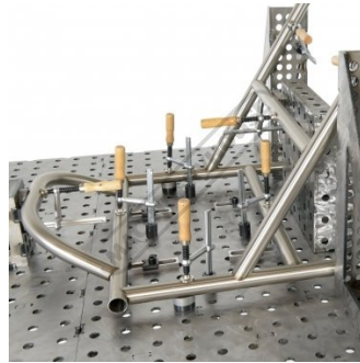
Shown With Optional Round Tube Framing Kit 9
