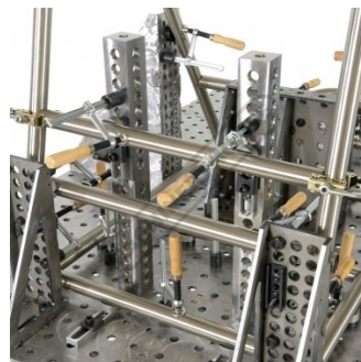
Shown With Optional Round Tube Framing Kit 6
