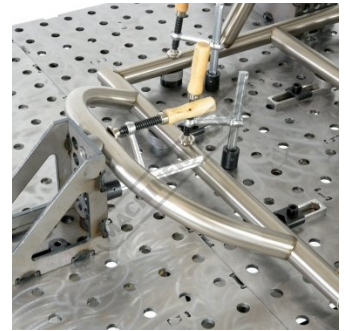
Shown With Optional Round Tube Framing Kit 11
